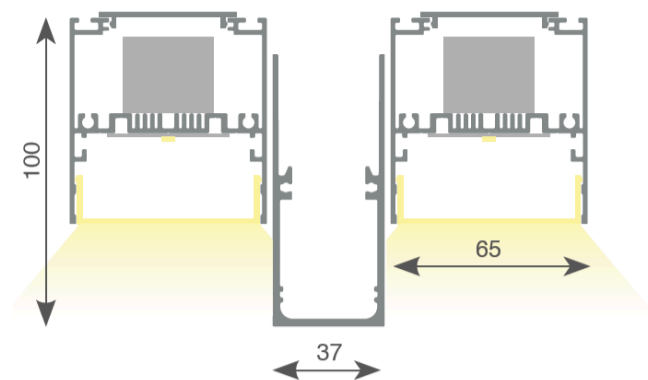
Prismatic diffusor
